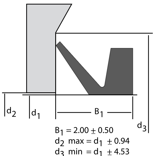
Assembly dimensions
