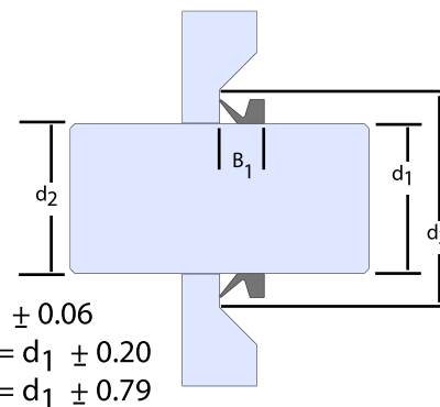
Assembly dimensions
