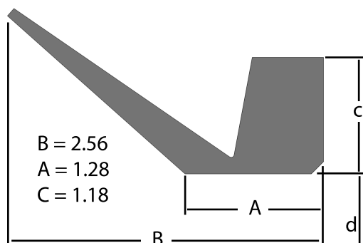
Profile dimensions
