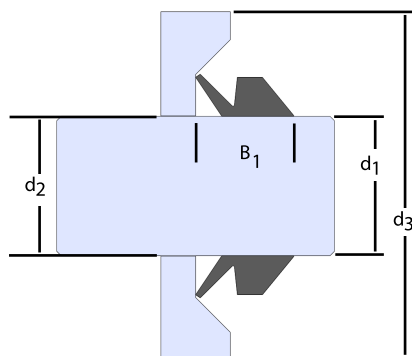
Assembly dimensions
